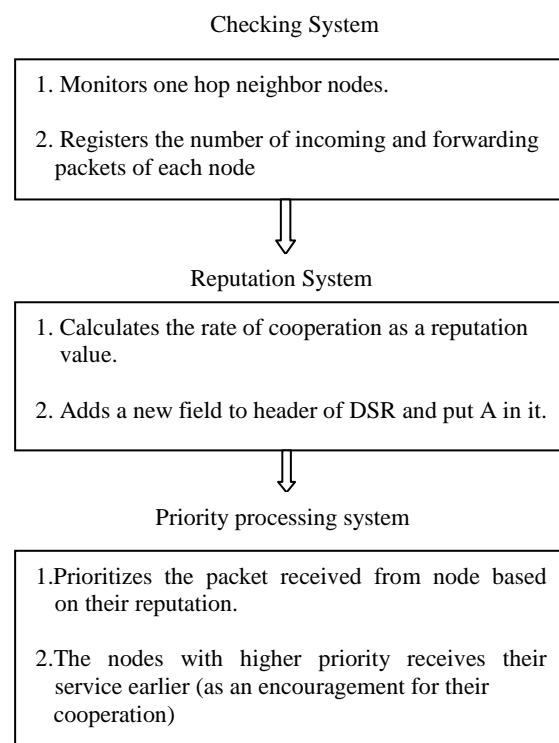
Figure 3: Process of reputation based mechanism to enforce cooperation in MANET
