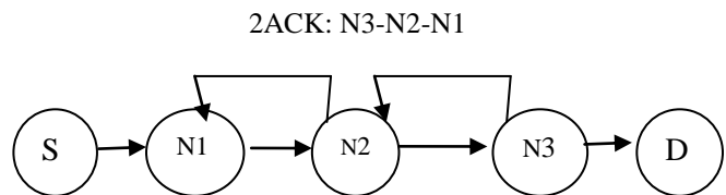
Figure 2: 2ACK Scheme
