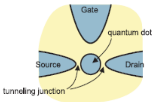
Fig. 8 Schematic structure of SET showing tunnel junctions.
