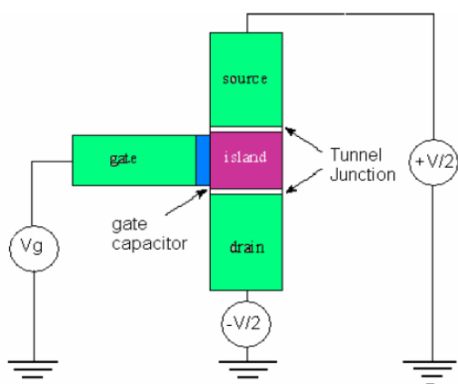
Fig. 5 Schematic structure of a SET
