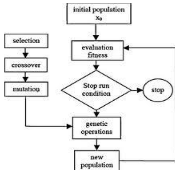
Flow Chart of Genetic Algorithm
