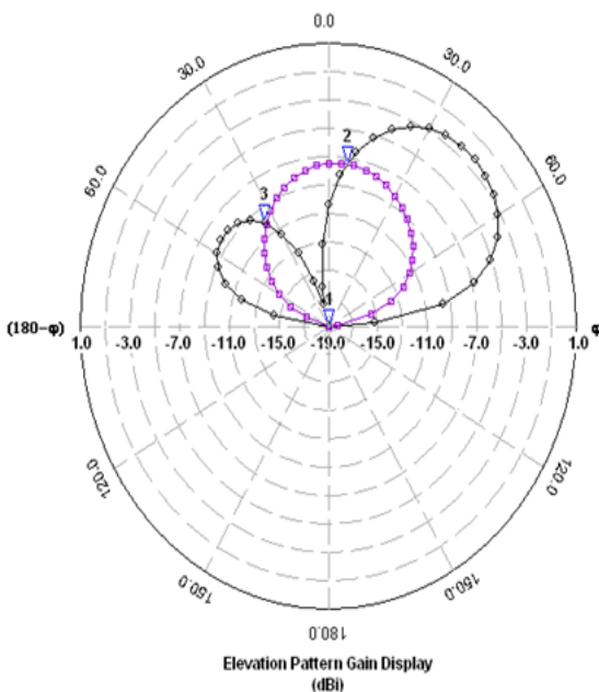
Figure 9: H-Plane Radiation Pattern for slotted antenna at 13.71 GHz
