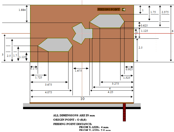
Figure 2: Simulated Antenna configuration
