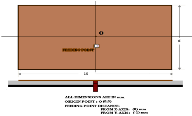
Figure 1: Conventional Antenna configuration
