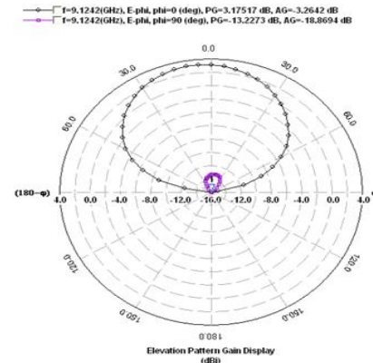
Figure 6: H-Plane Radiation Pattern for slotted Antenna at 9.1242 GHz
