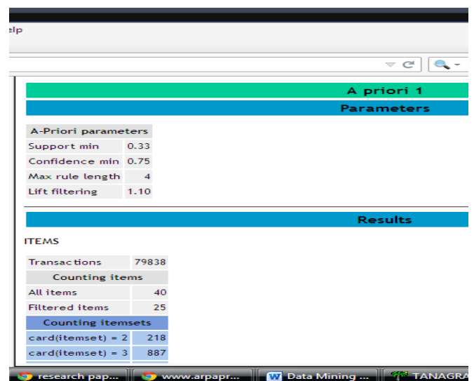
Figure 2 Association rule mining graph using TANAGRA tool
