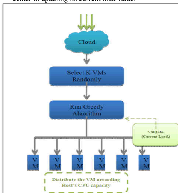
Figure 2 the Proposed Algorithm
