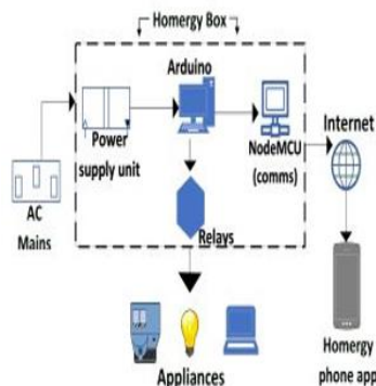
Fig. 3: General System Architecture
