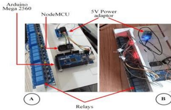
Fig. 6: Internals of Homergy Box with (B) and without (A) Relay Wiring
