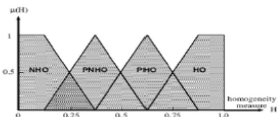
Fig. 6. The fuzzy sets used for homogeneity inference.
