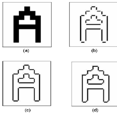
Fig. 5. The comparison of the edge detections for the example image.
