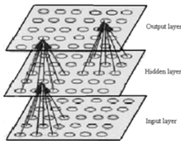
Fig. 8. Neural network approach for Image Segmentation Process
