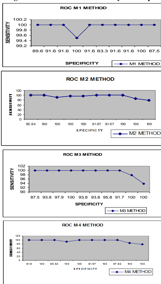
Figure 5: ROC Measures of Four SDT Post classifiers
