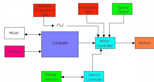
Figure 1: The control system
