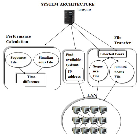
Fig 8.1: System Architecture
