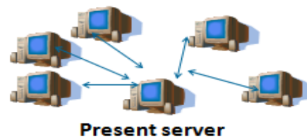
Fig 3.1: Unidirectional Peer-to-peer
