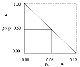
Fig 3.1 Wall Static Pressure Variation M.F For Nozzle with mach no - 1.58
