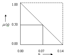
Fig 3.3 Wall Static Pressure Variation M.F For Nozzle with mach no - 2.06
