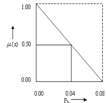
Fig 3.4 Wall Static Pressure Variation M.F For Nozzle with mach no - 2.23
