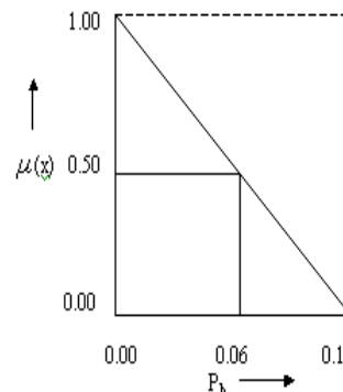
Fig 3.1 Wall Static Pressure Variation M.F For Nozzle with mach no - 1.58
