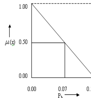
Fig 3.3 Wall Static Pressure Variation M.F For Nozzle with mach no - 2.06
