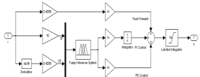
Figure 3. Simulation of Fuzzy PID Controller
