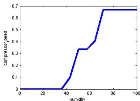
Fig.9. Compressor speed with humidity
