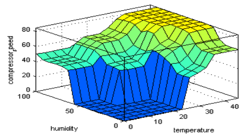
Fig.4. Surface view of Mamdani-type FIS
