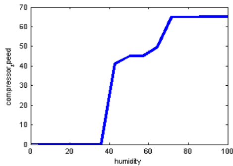
Fig.6. Compressor speed with humidity
