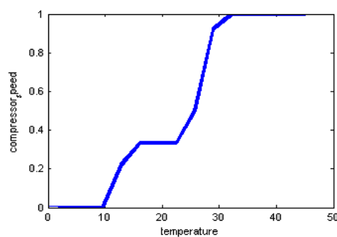
Fig.8. Compressor speed with temperature
