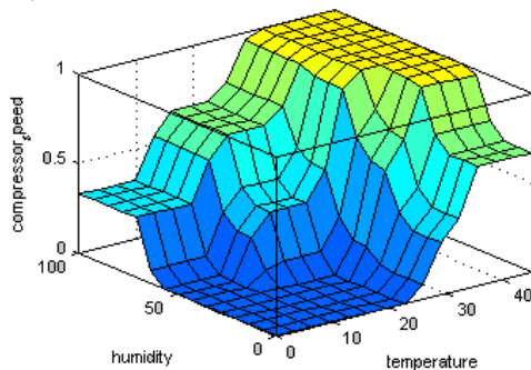
Fig.7. Surface view of Sugeno-type FIS
