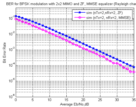
Figure 1: BER plot for 2x2 MIMO with ZF receiver (Top) and MMSE (Below) for BPSK modulation in Rayleigh channel.
