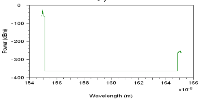
Fig 3.4 Wavelength spectrum of A = '1' & B = '0'
