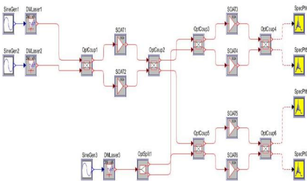
Schematic diagram of encoder (A = '1', B = '1')
