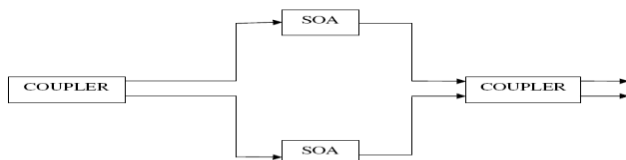
Fig 3.1 Optical logic using MZI switch
