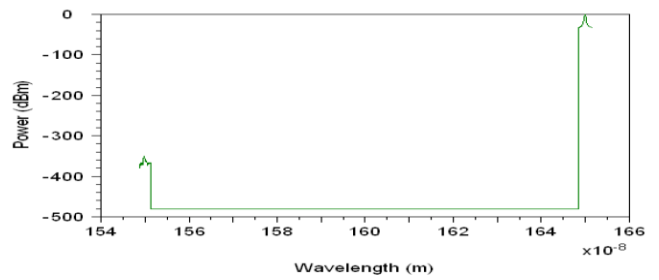
Wavelength spectrum of A = '1' & B = '1'
