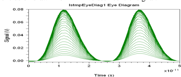
Fig 4.4 Eye Diagram
