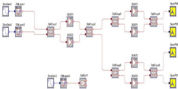
Fig 3.3 Schematic Diagram of Multiplexer (A = '1', B = '0')
