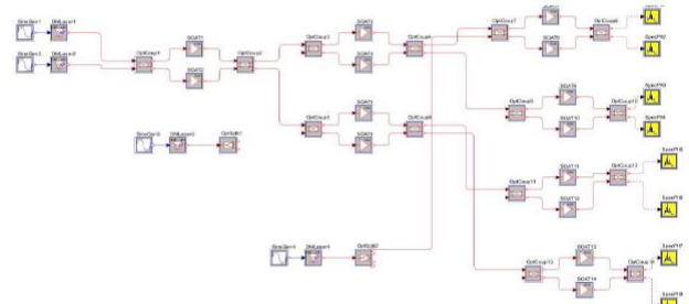
Schematic diagram of encoder (A = '1', B = '0', EN='1')
