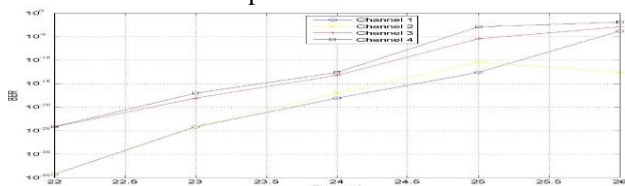
Fig 4.3 BER versus power control signal with dispersion
