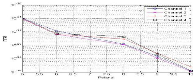
Fig 4.2 BER versus input signal power with dispersion
