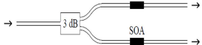
Fig 1.4 SOA based MZI Switch
