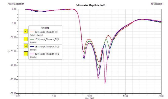
Fig.11 S11 of various size of S_b
