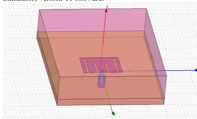
Figure 1: Design of E+U shaped patch antenna
