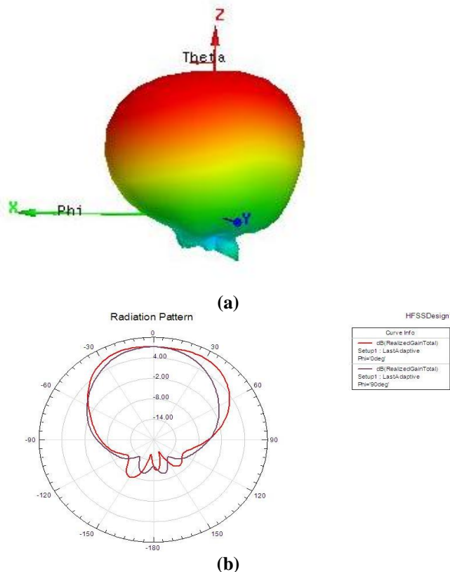
Fig. 14(a) & (b) 8.73 GHz radiation pattern
