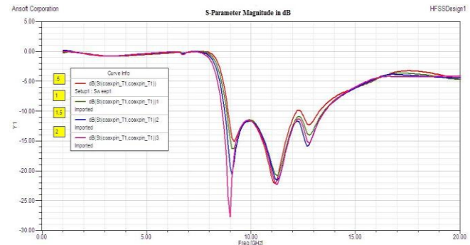
Fig.10 S11 of various size of S_a
