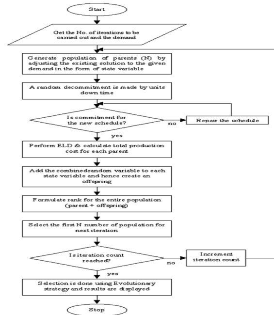
Fig. 1 Flow Chart for UCP using EP
