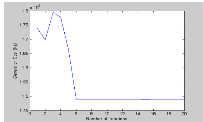
Fig. 3 Cost Convergence Characteristics for 20 Iterations
