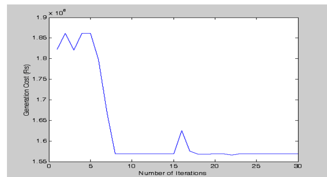
Fig. 4 Cost Convergence Characteristics for 30 Iterations
