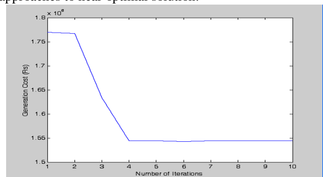
Fig. 2 Cost Convergence Characteristics for 10 Iterations
