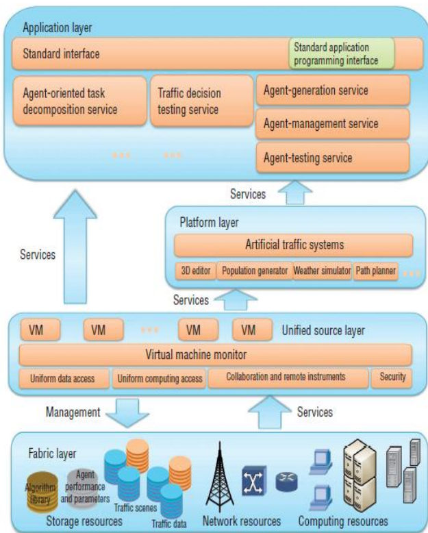
Fig. 5 Intelligent traffic clouds have fabric, unified source layer, platform and application layers.
