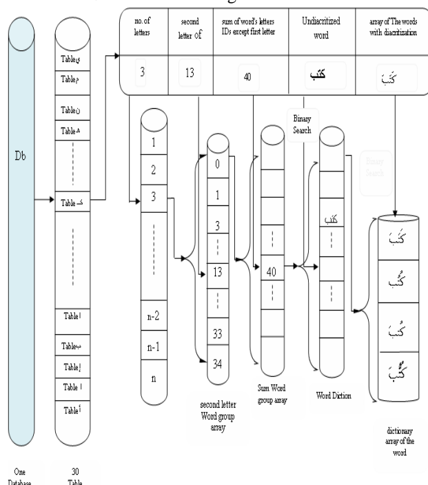
Fig3: shows how the word "كتب" is found in the dictionary.
