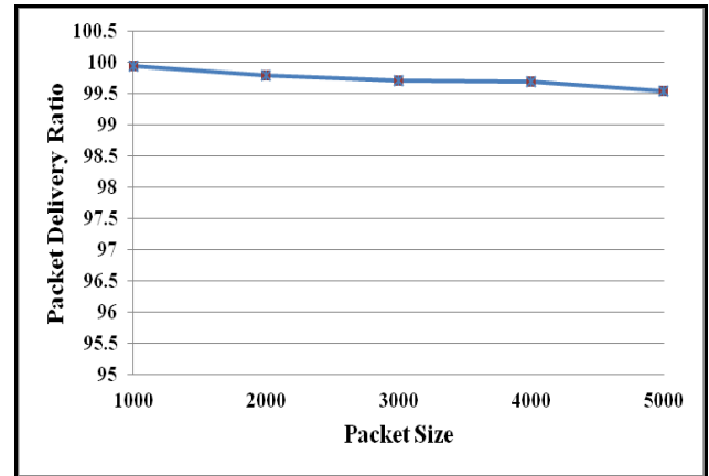
Figure 12: Packet Delivery Ratio vs. Packet Size
