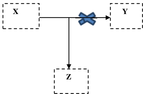
Figure 1 Impersonation Attack
