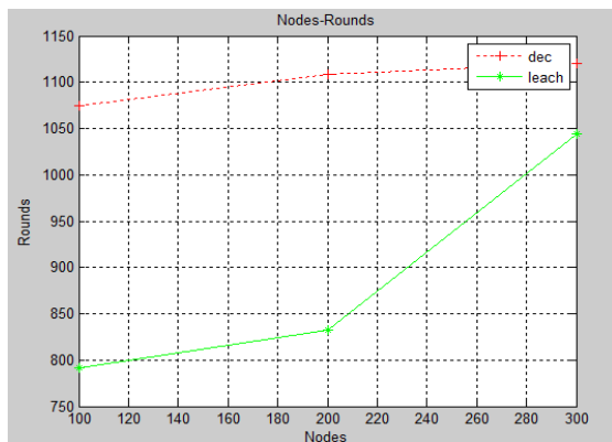
Figure 8: Nodes with respect to number of rounds considering packet length of 8400 bytes
