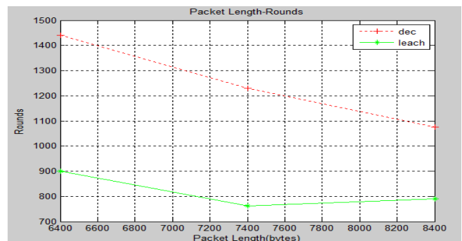
Figure 5: Packet length with respect to number of rounds considering 100 nodes
