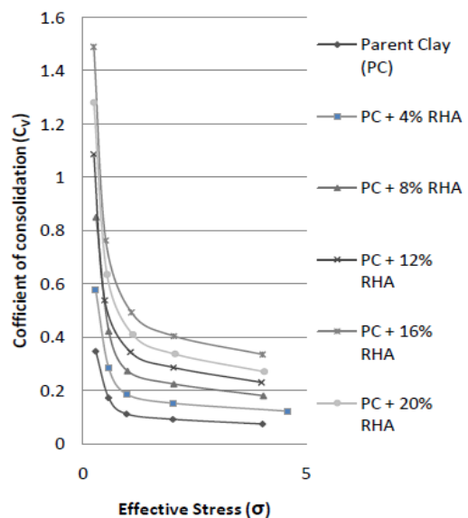
Figure 3. Variation of coefficient of consolidation with effective stress for various percentages of rice husk ash
