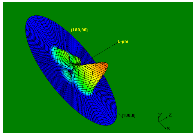
Figure 12: H-Plane Radiation Pattern for slotted antenna at 13.71 GHz
