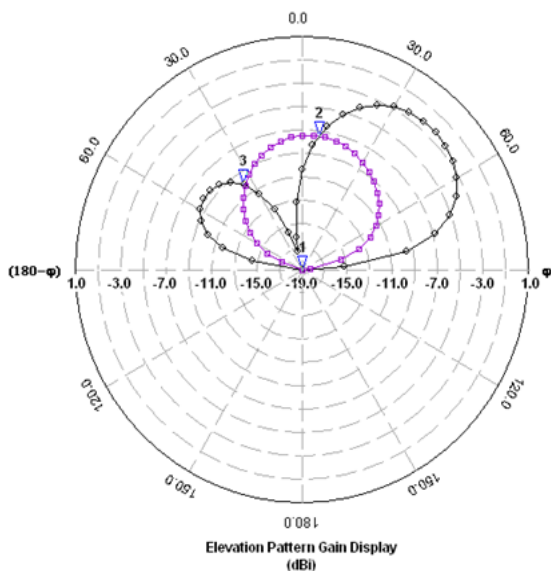
Figure 9: H-Plane Radiation Pattern for slotted antenna at 13.71 GHz
