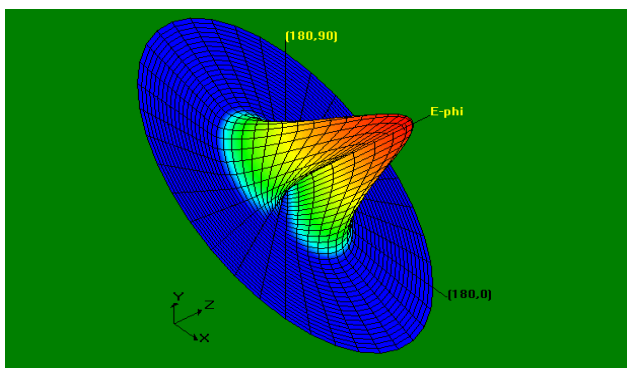
Figure 8: H-Plane Radiation Pattern (3D) for slotted antenna at 9.12 GHz
