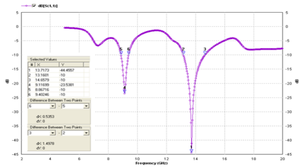
Figure 4: Return Loss vs. Frequency (Slotted Antenna)
