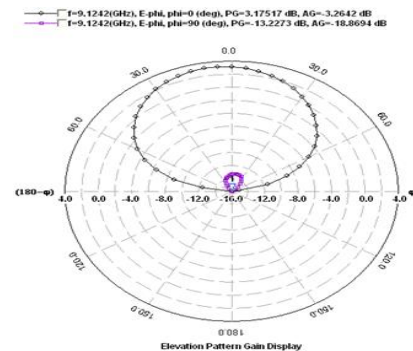
Figure 6: H-Plane Radiation Pattern for slotted Antenna at 9.1242 GHz
