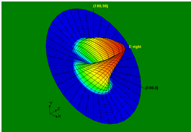
Figure 7: E-Plane Radiation Pattern (3D) for slotted antenna at 9.12 GHz
