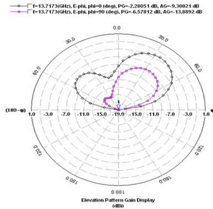
Figure 10: H-Plane Radiation Pattern for slotted antenna at 13.71 GHz
