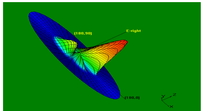
Figure 11: E-Plane Radiation Pattern for slotted antenna at 13.71 GHz
