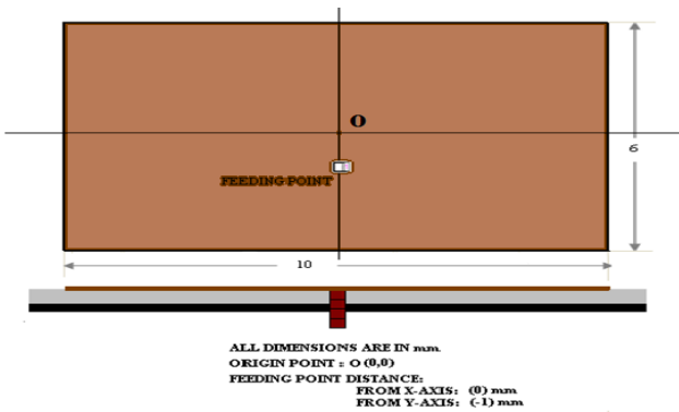
Figure 1: Conventional Antenna configuration
