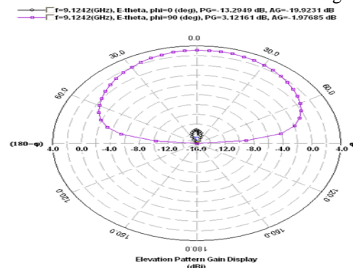
Figure 5: E-Plane Radiation Pattern for slotted Antenna at 9.1242 GHz
