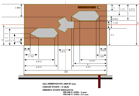
Figure 2: Simulated Antenna configuration
