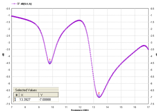
Figure 3: Return Loss vs. Frequency (Conventional Antenna)
