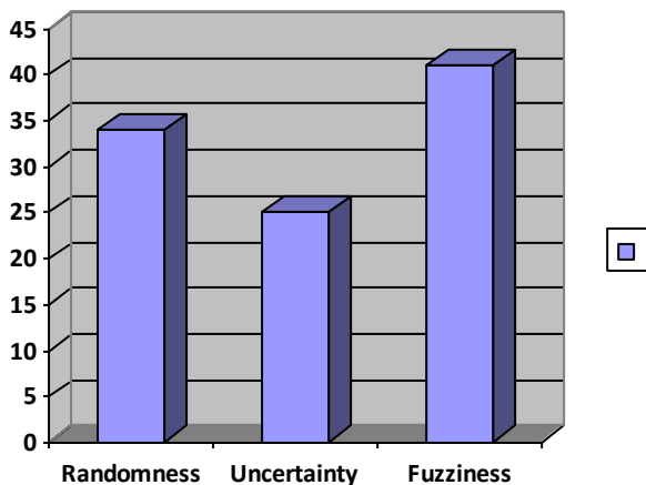
Fig. 4: Performance analysis chart for Optimum deception detection Rate Percentage
