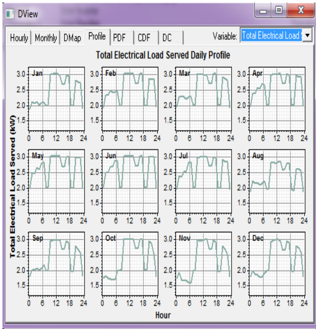
Fig 17 Total electrical lode served daily profile
