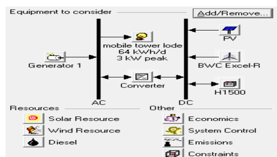
Fig.1 system implementation in Homer ( PV-Photovoltaic, BWC Excel-R-Wind turbine, H1500-Battery, Generator 1- Diesel generator
