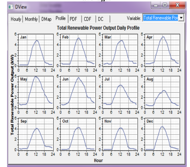
Fig 16 Total renewable power output daily profile
