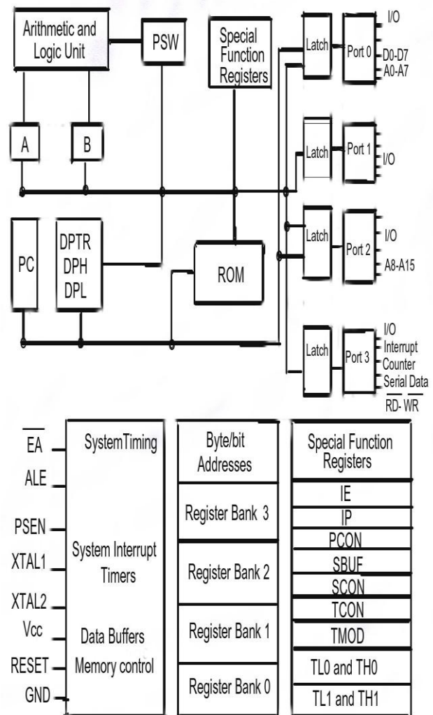
Fig.5 Block diagram of microcontroller 89c51
