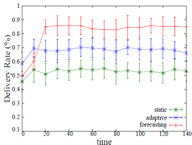
Fig. 4. Packet Delivery Rate over Periodically Unreliable Links
