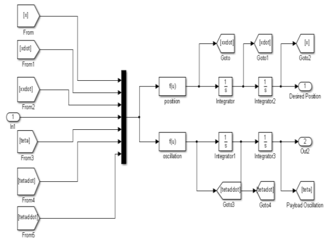
Fig. 4: Subsystem in the gantry crane system
